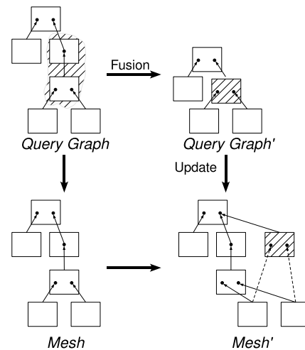
Figure 11: Updating the mesh
