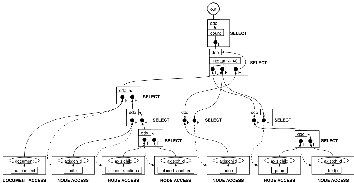
Figure 3: Query graph after translation
