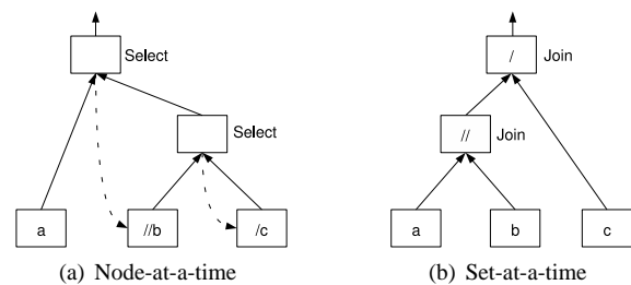
Figure 2: Evaluation strategies for XML queries
